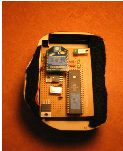
Figure 2. The Transmitter Circuit
